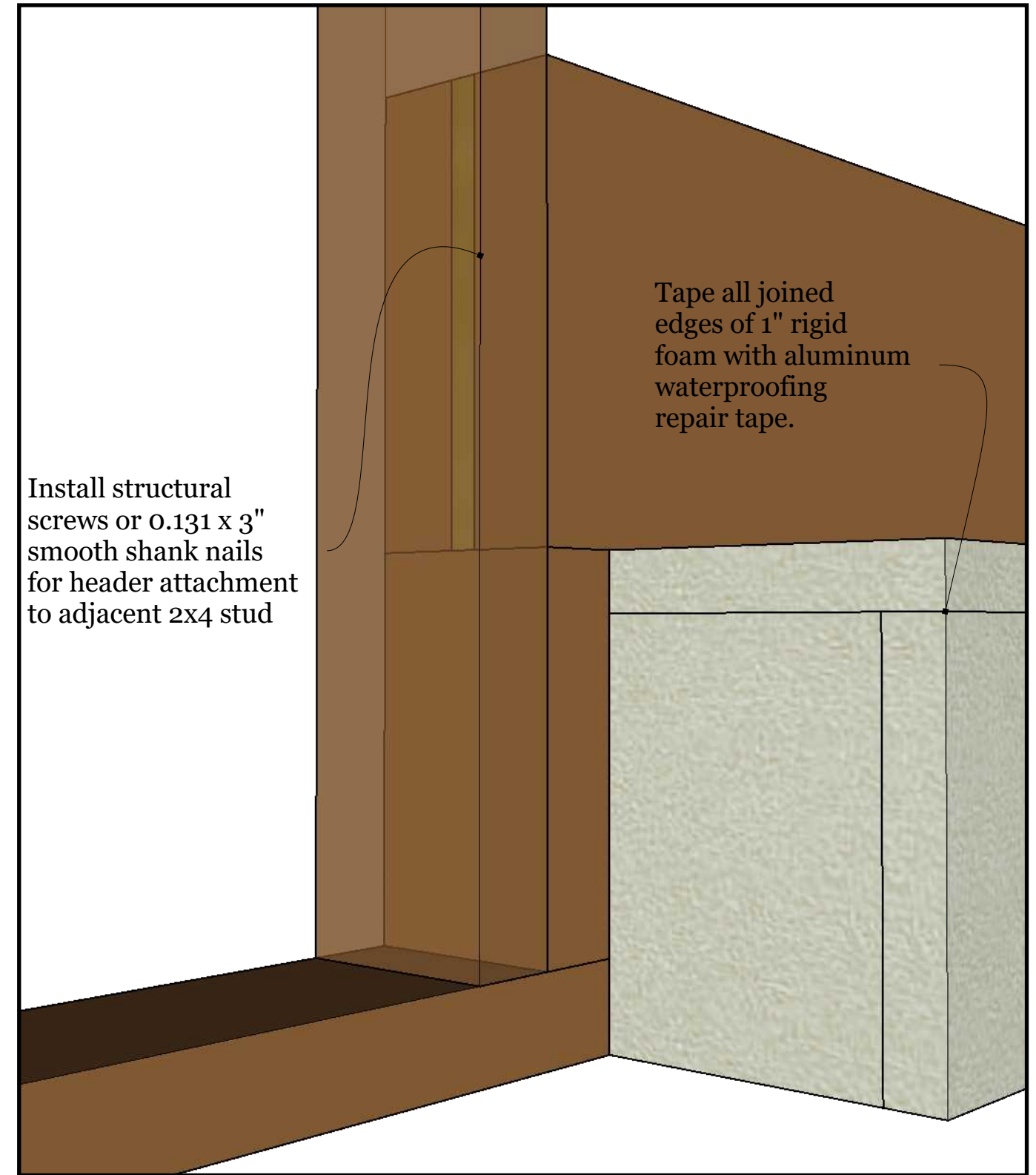
Detail #2 - Wheel Well Header 2
