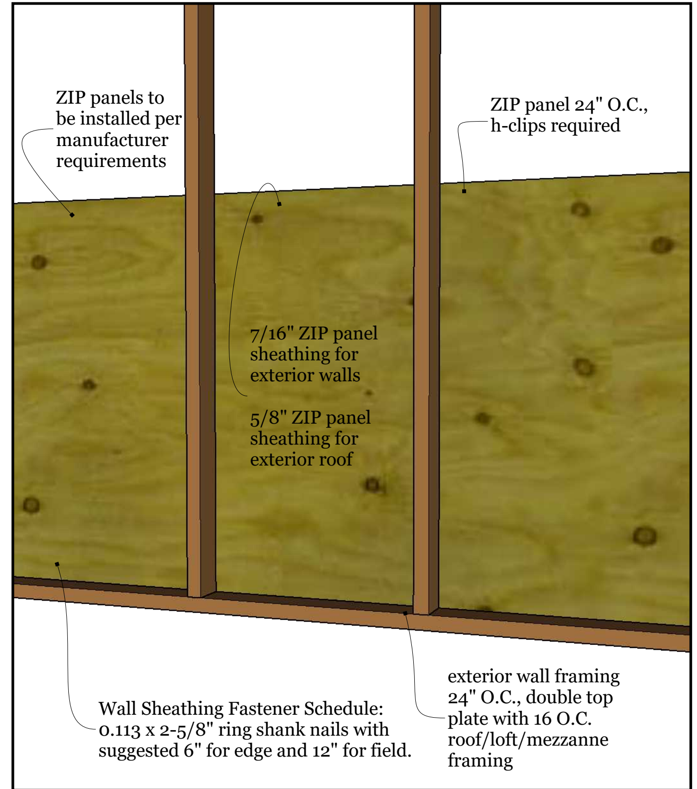
Detail #9 - Sheathing & Fastener Schedule
