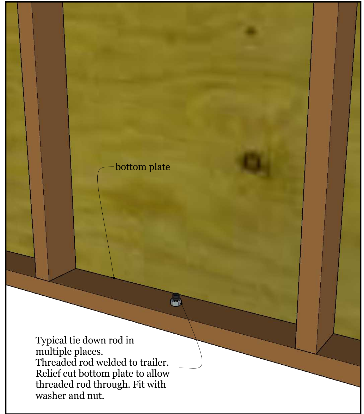
Detail #4 - Tie Down
