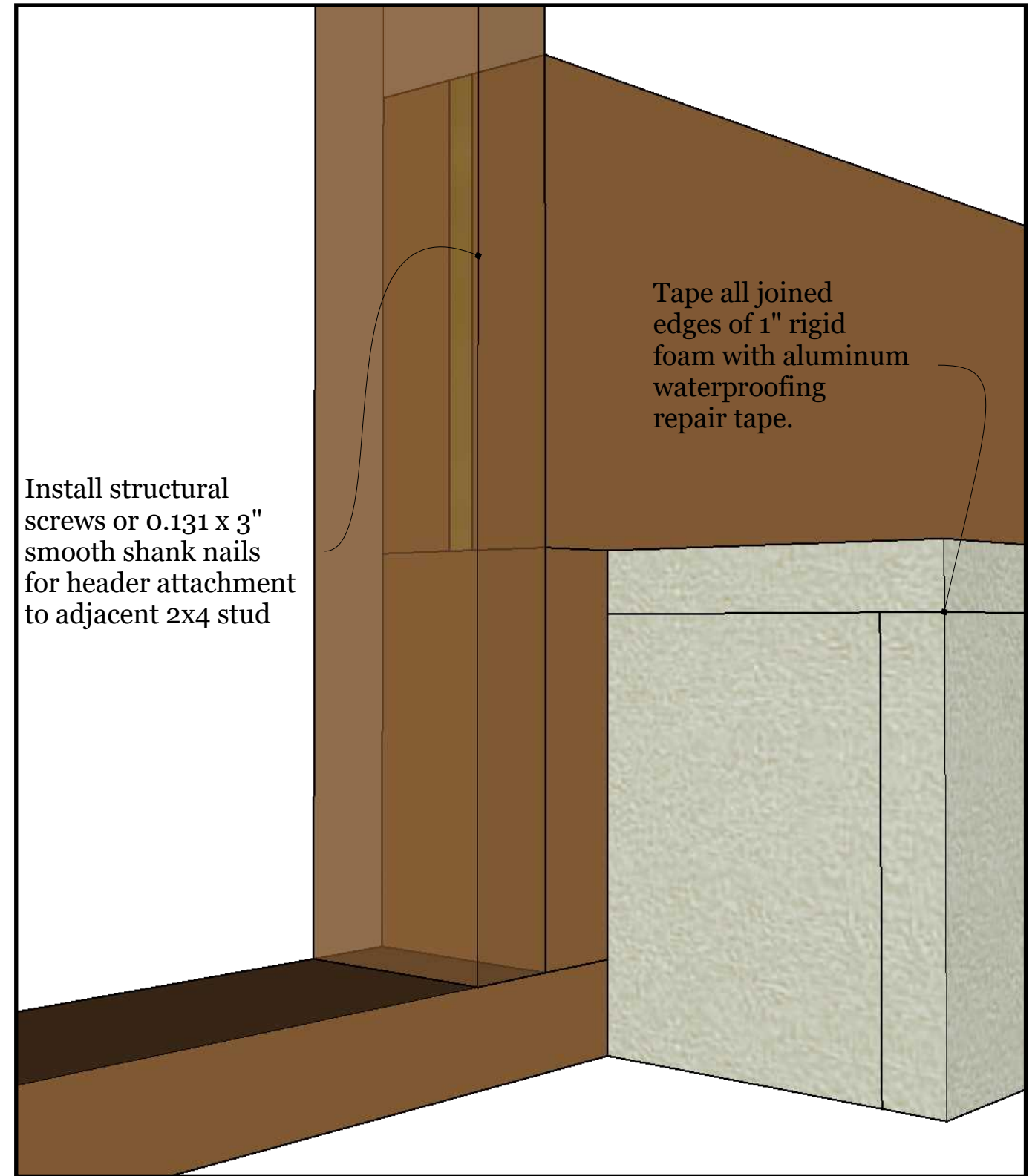
Detail #2 - Wheel Well Header 2
