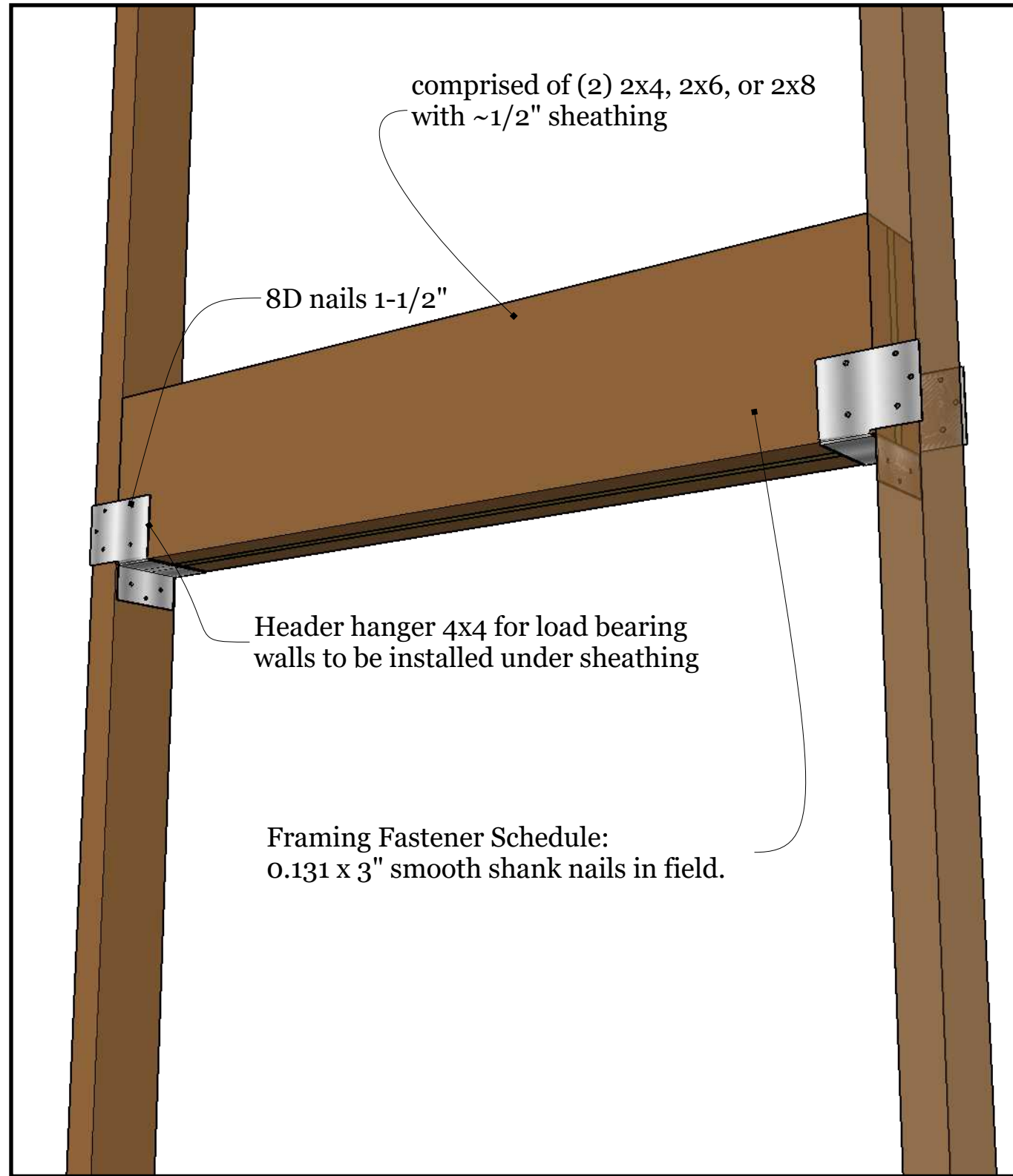
Detail #3 - Window/Door/Opening Header
