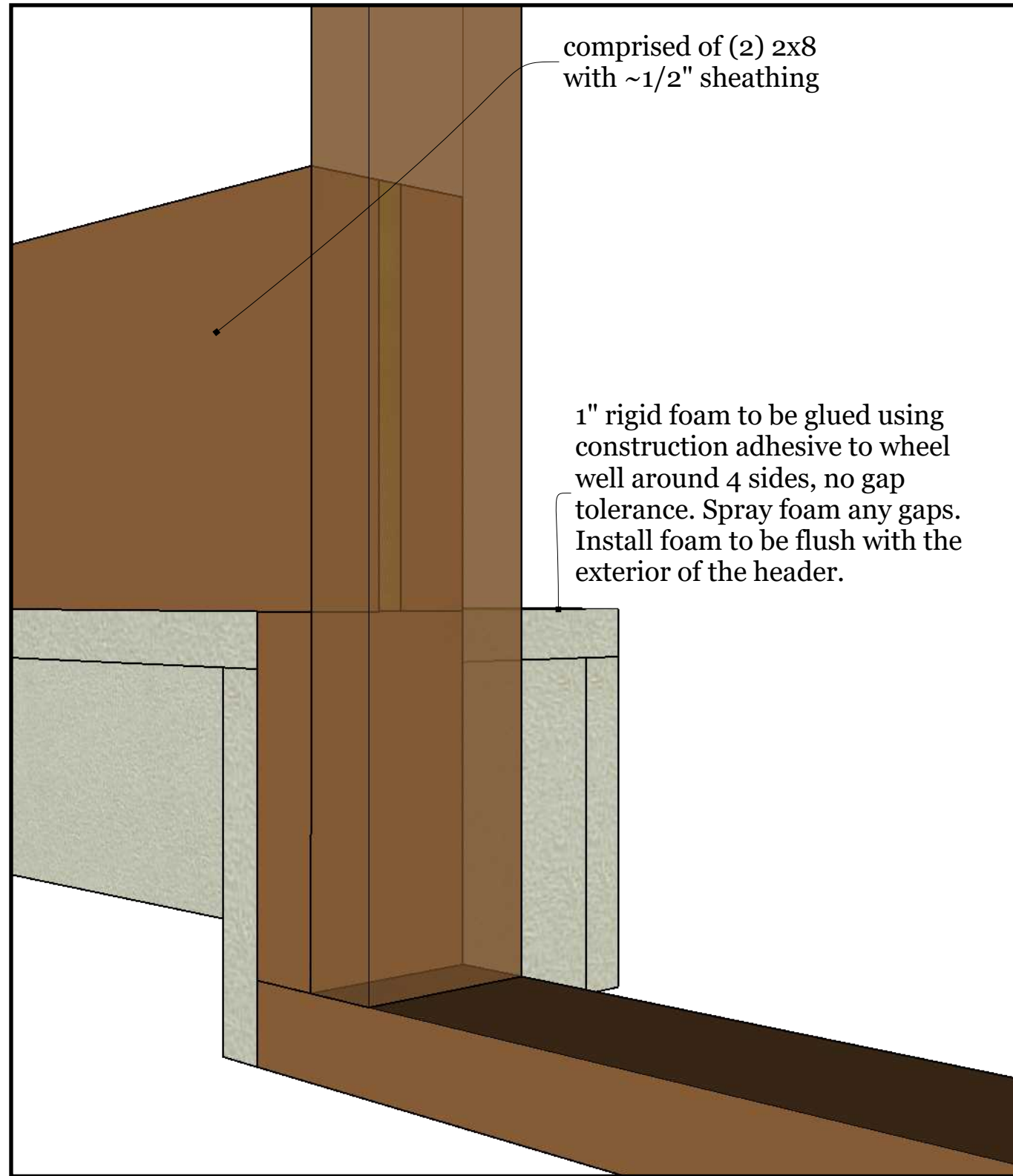
Detail #1 - Wheel Well Header 1
