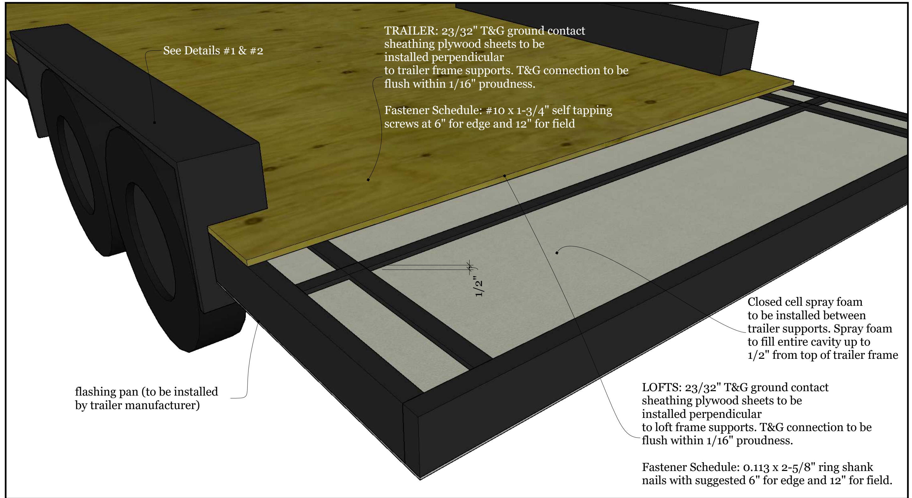
Detail #7 - Trailer & Loft Subfloor
