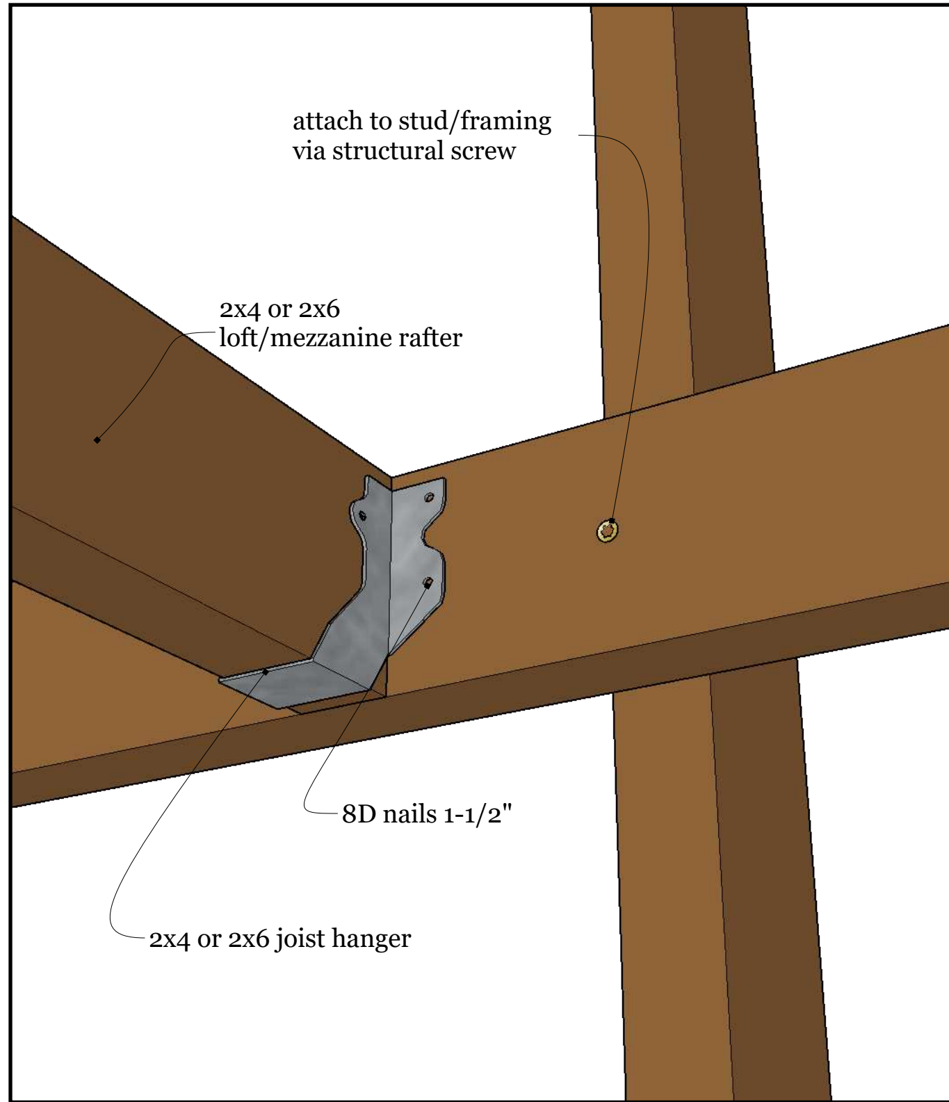
Detail #5 - Loft/Mezzanine Tie (supported)
