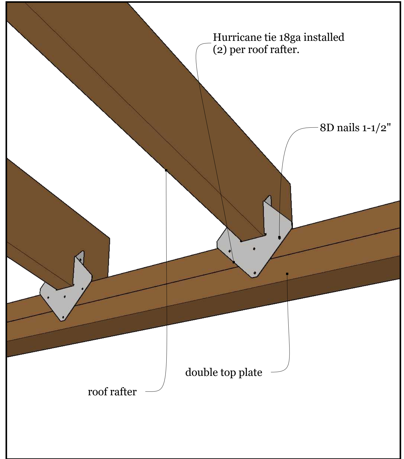
Detail #6 - Roof Rafter Tie
