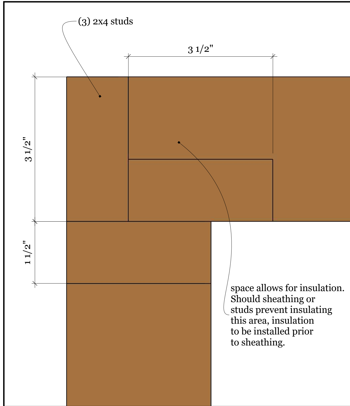
Detail #8 - California Corner
